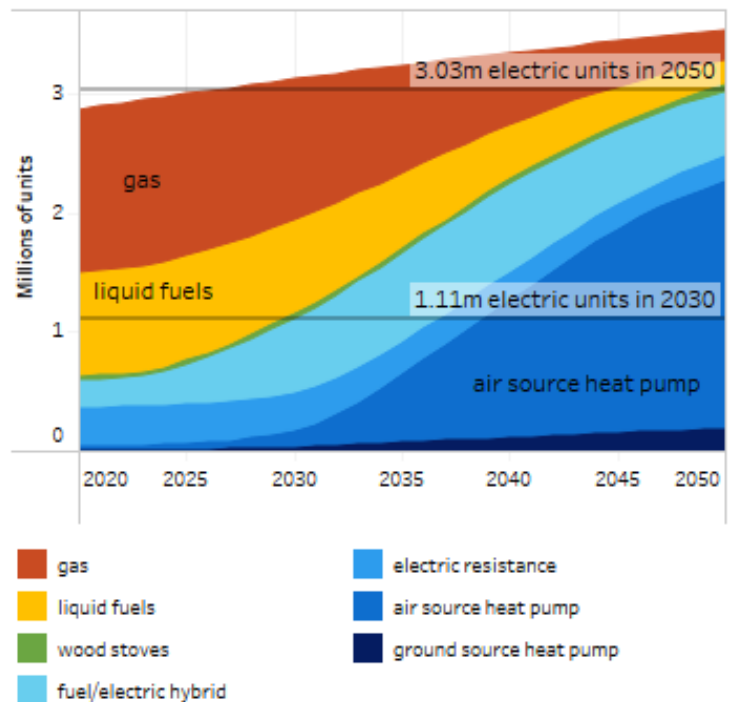
Figure 3.2. Residential Space Heating Stock, Phased Scenario
